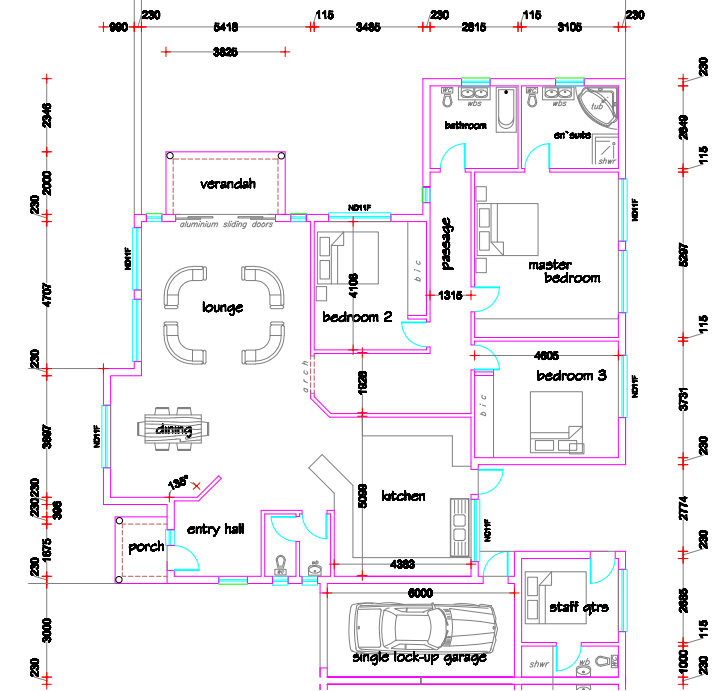
Unit Floor Plan
